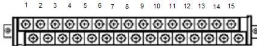
Figure 21 Terminal # 1 Pin Configuration
