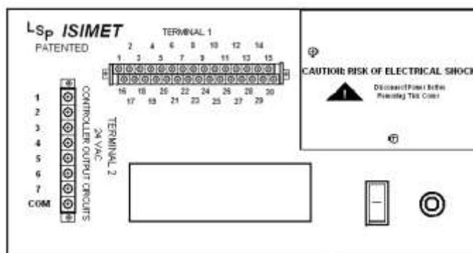
Figure 3 - 24 VAC Control Panel
