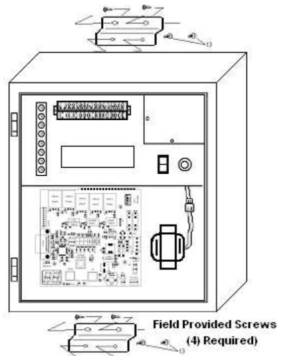
Figure 7 - Surface Mounted
