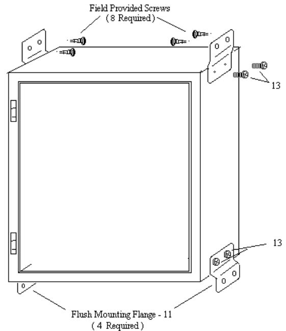
Figure 2 For best Flush Mounting results, recess face of enclosure's lip 1/2" behind wall finish
